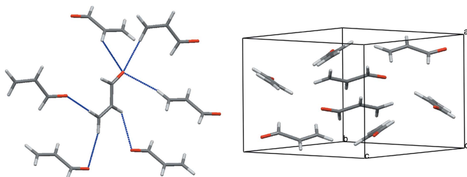
Figure 1 Packing diagrams of the crystal structure of molecule (XII). Grey = carbon, white = hydrogen, red = oxygen. C-H \cdots O contacts (with R_{O \cdots H} shorter than the sum of van der Waals radii) are indicated as blue lines.
